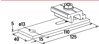
SSP Speed Plus 12 A2
